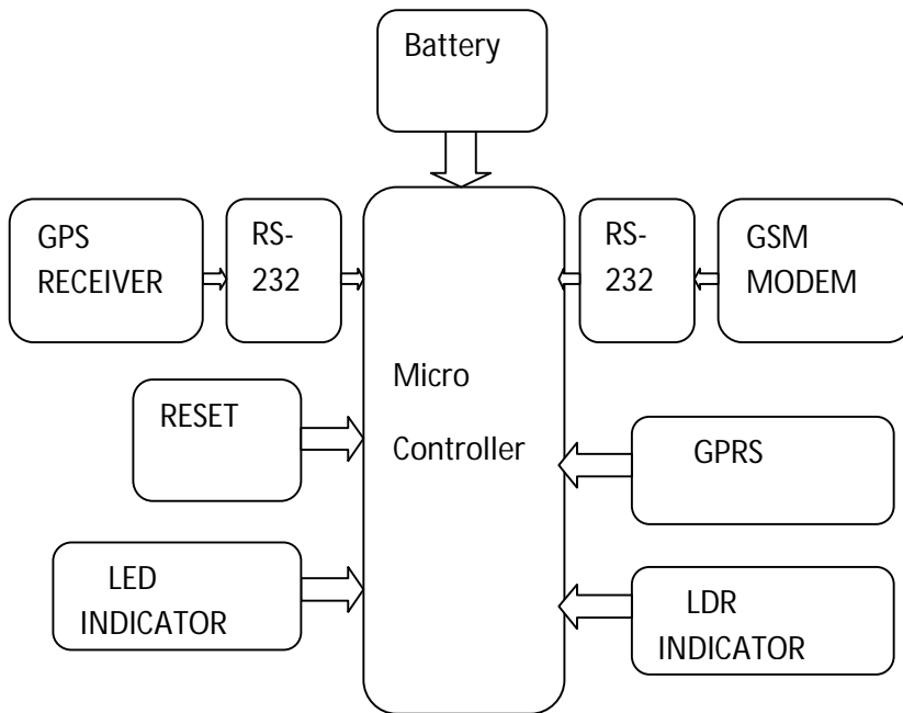
Fig.4 Automatic Broken Rail Detection Scheme using LED-LDR Assembly
