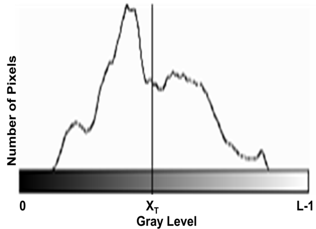
Fig. 1 Bi-histogram equalization
