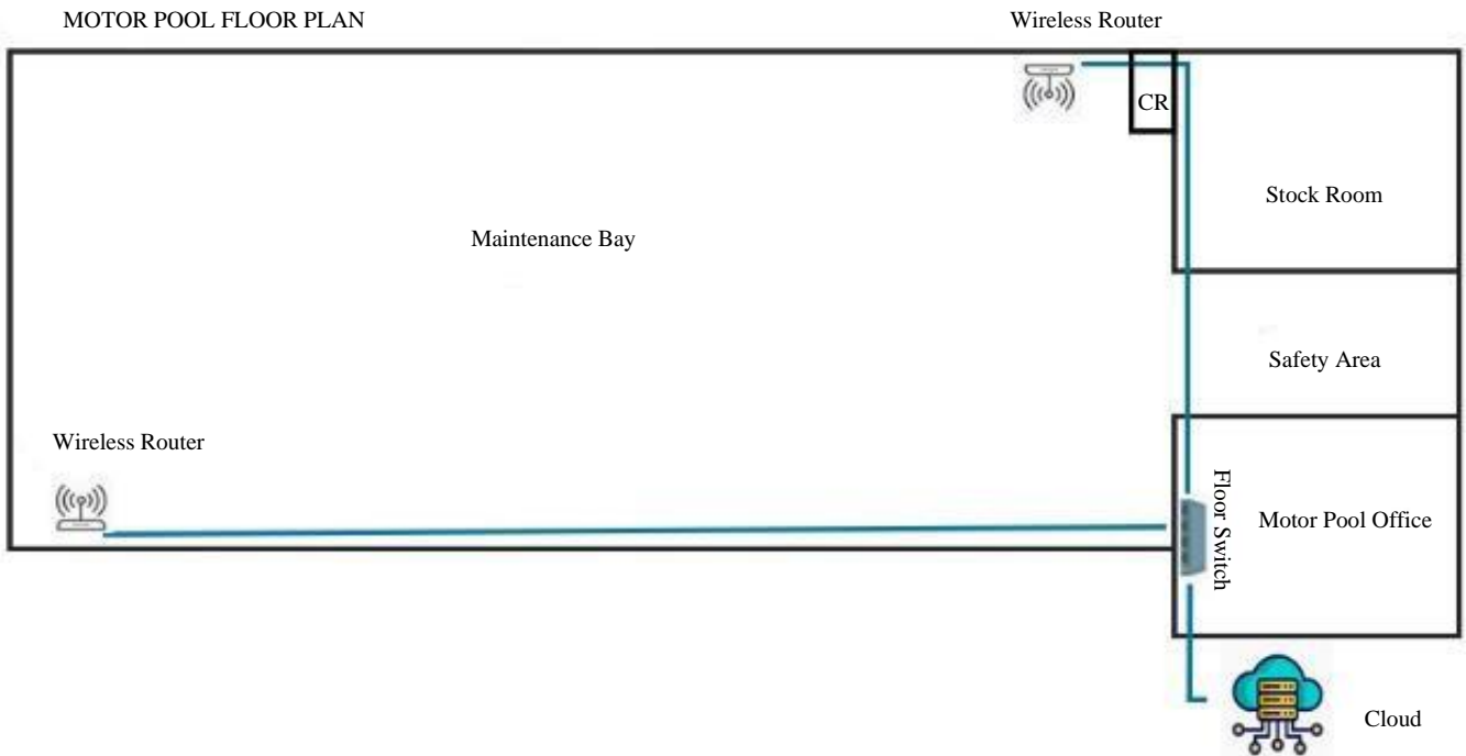
Fig. 14 Physical network design for Motor Pool
