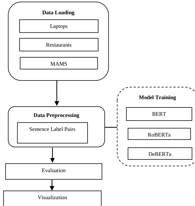
Fig. 1 Proposed architecture
