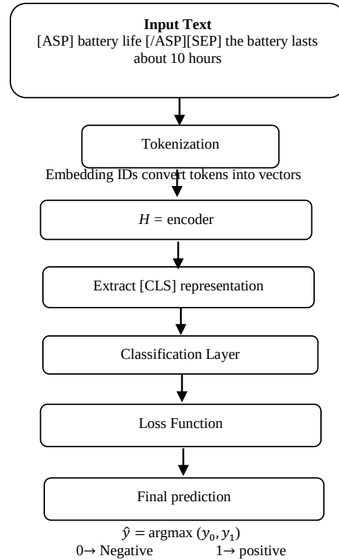
Fig. 4 DeBERTa-base architecture
