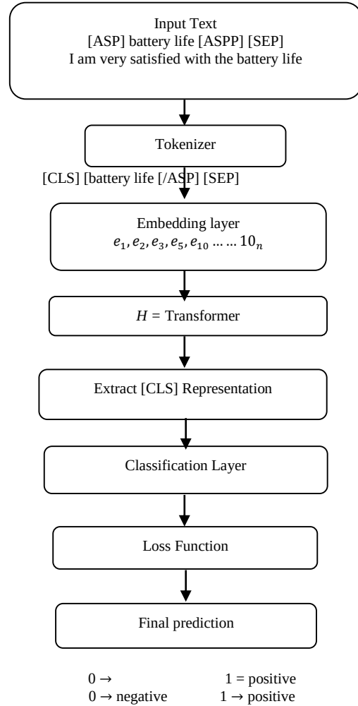
Fig. 2 BERT-base-uncased architecture
