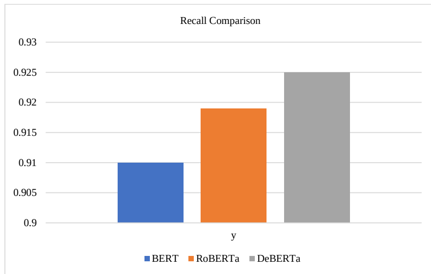
Fig. 7 Recall performance comparison
