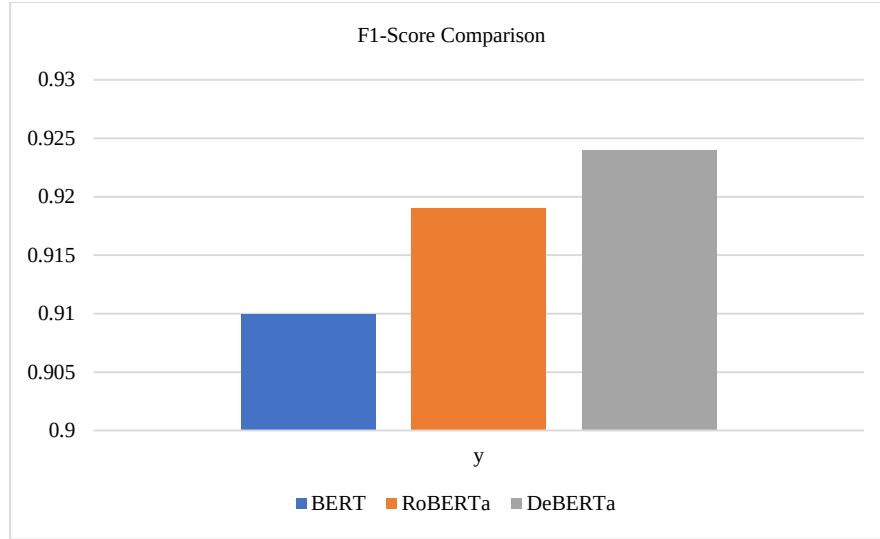
Fig. 8 F1-Score performance comparison
