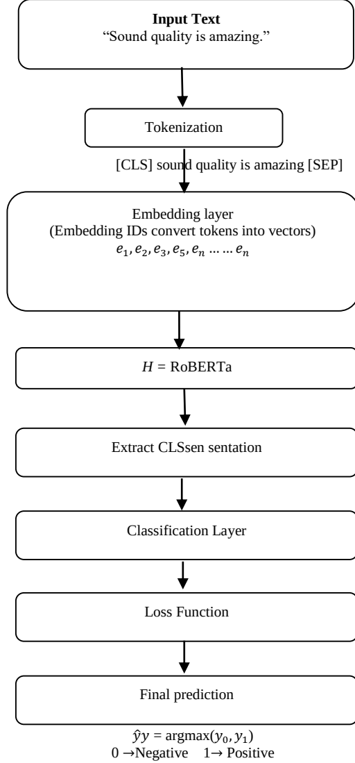
Fig. 3 RoBERTa-base architecture
