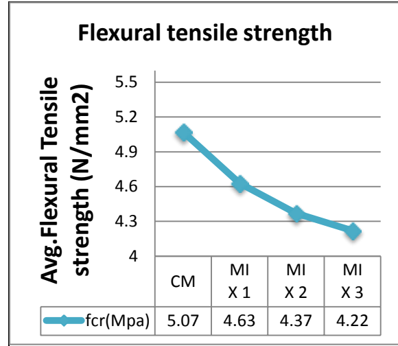
Fig.4 Flexural tensile strength
