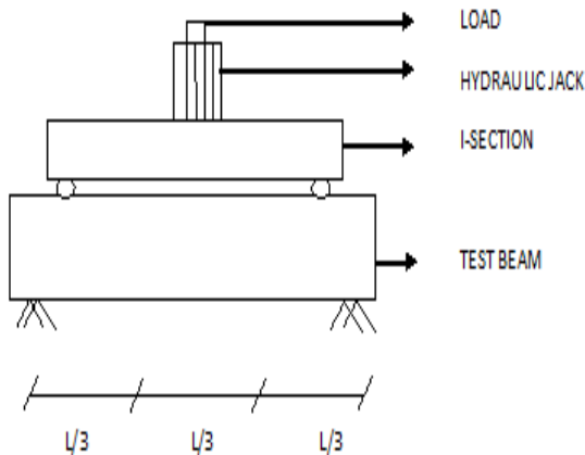
Fig.3 Test Setup
