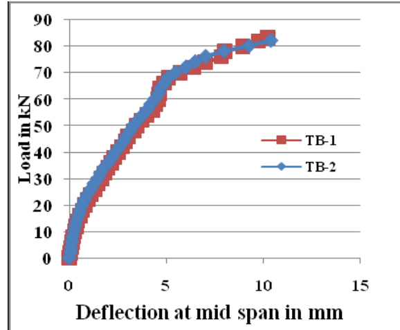
Fig.5 Deflection at mid span
