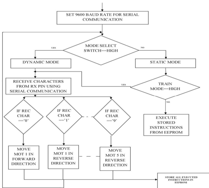
Fig.6 Receiver Flow Chart
