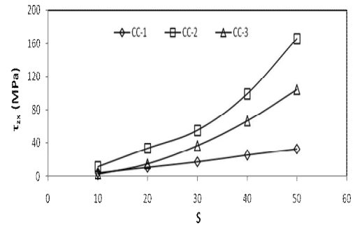
Fig 11: Variation of \tau_{zx} with 's' in I-2
