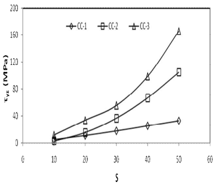
Fig 8: Variation of \tau_{yz} with 's' in I-2
