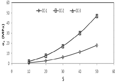
Fig 6: Variation of \sigma_z with 's' in I-3
