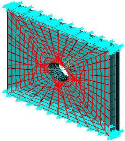
Figure 3 : FE model with CC-3
