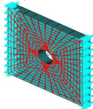
Figure 2 : FE model with CC-2
