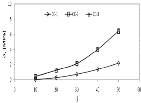
Fig 5: Variation of \sigma_z with 's' in I-2
