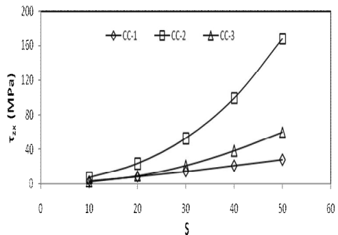
Fig 12: Variation of \tau_{zx} with 's' in I-3
