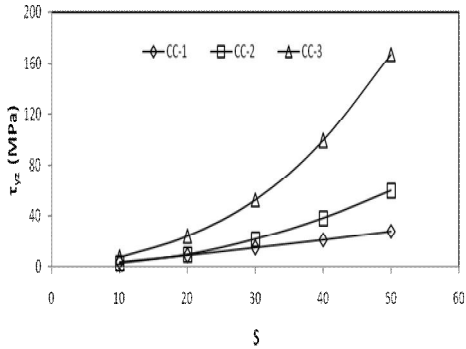
Fig 7: Variation of \tau_{yz} with 's' in I-1
