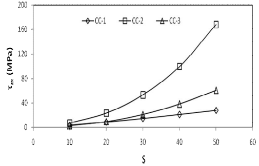
Fig 10: Variation of \tau_{zx} with 's' in I-1
