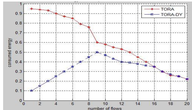
Fig.2. Energy consumption for variable flows
