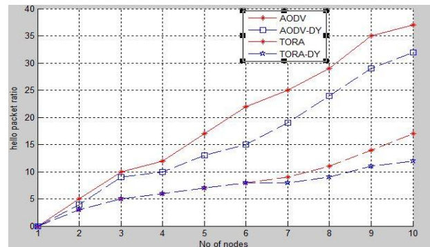
Fig.3. Hello packet overhead
