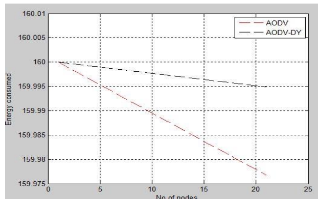
Fig.4. Energy consumption for AODV
