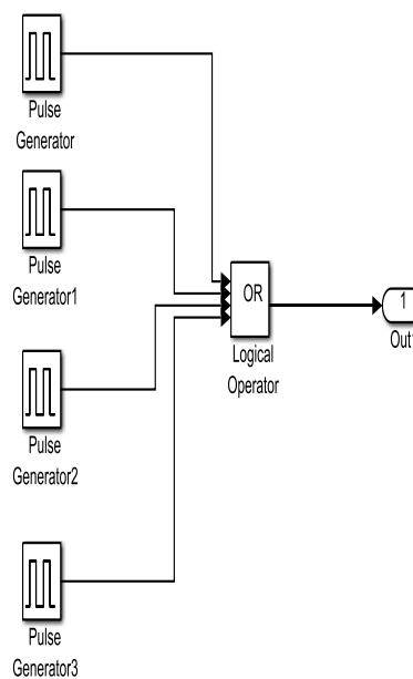
Figure 5. Subsystem of Generating Pulses
