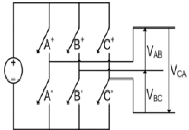
Figure 2. Topology of a Basic Three Phase Inverter
