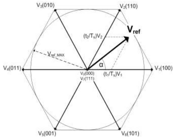
Figure 3. Vector Representation of SVM
