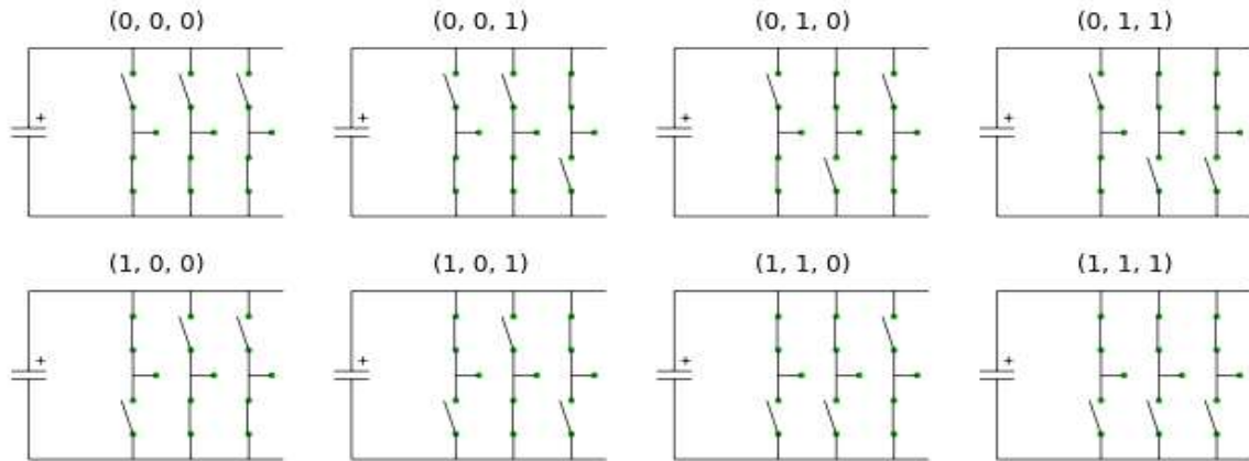
Figure 4. Eight possible Switching States
