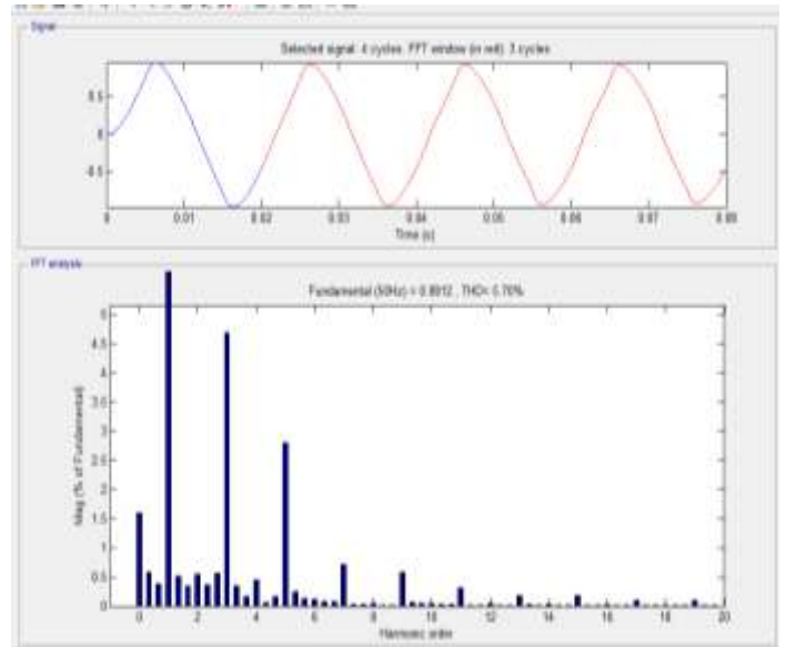
Figure 9. Harmonic Spectrum (THD 5.70%)
