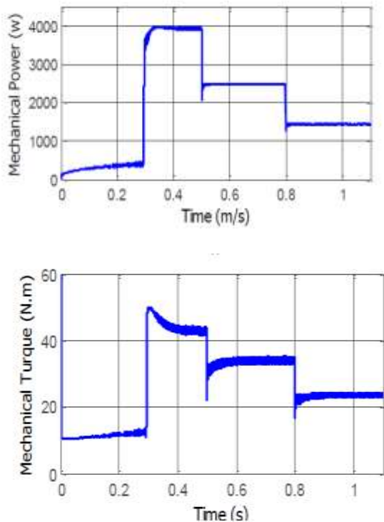
Fig. 10. (a) the mechanical power and (b) turbine torque curves
