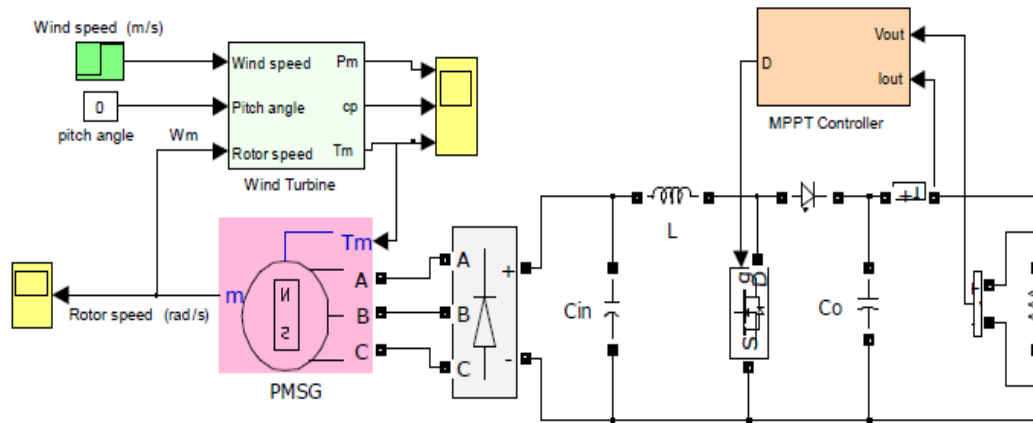
Fig. 4. Schematic of wind generation system
