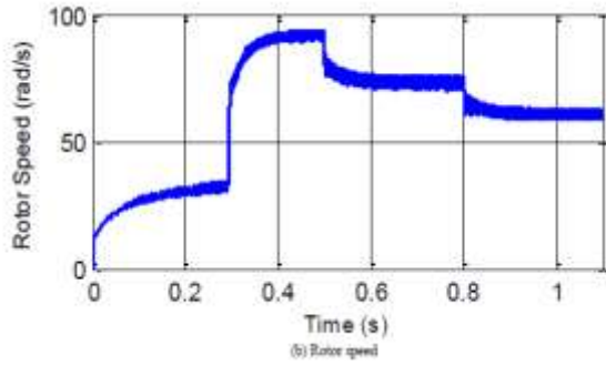
Fig. 8. Simulation results of rotor speed for a step variation of wind speed.
