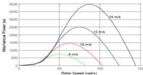
Fig. 2. The power curves for different wind speeds and zero pitch angle
