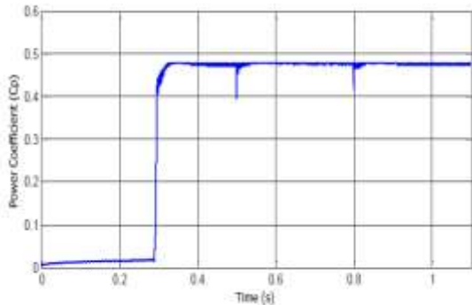
Fig.9. Simulation results of aerodynamic constant Cp for three step variation of wind speed
