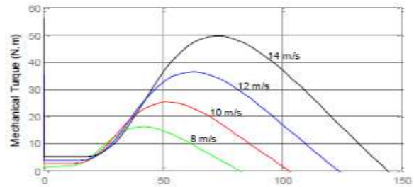
Fig. 3. The Torque curves for different wind speeds and zero pitch angle
