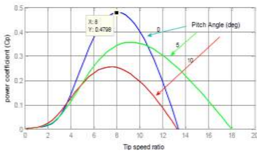
Fig.1. Wind-turbine power coefficient characteristics of a wind turbine.
