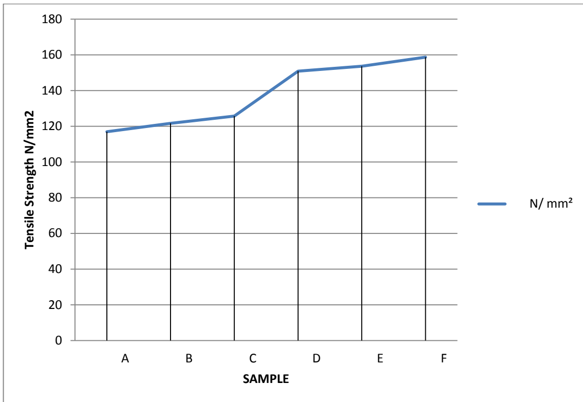
Fig 1.2. Graph for the tensile strength for each sample
