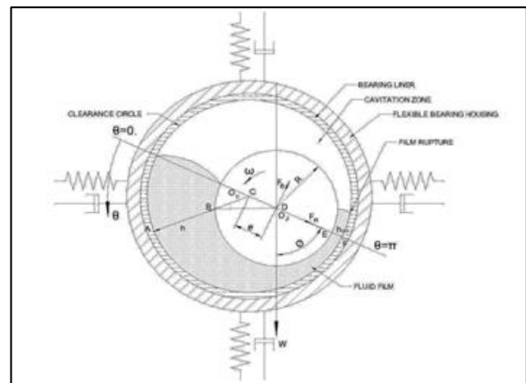
Fig. 1: shows the schematic diagram of the flexibly supported oil journal bearing with flexible liner:
